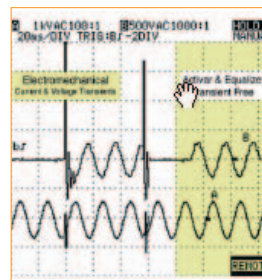
Electromechanical vs. Transient-free switching
