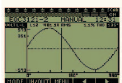
Waveform Display
