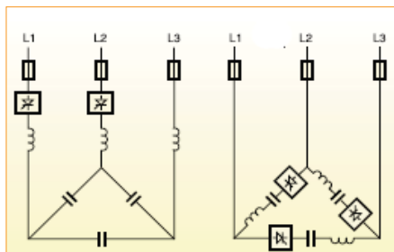
2 & 3 phase Switching Structure
