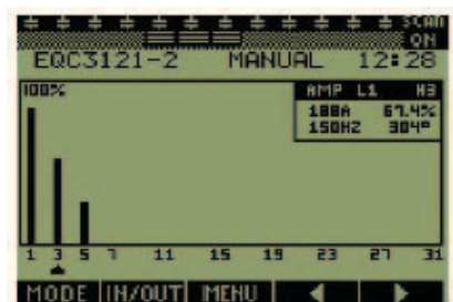
Harmonic Bar Display
